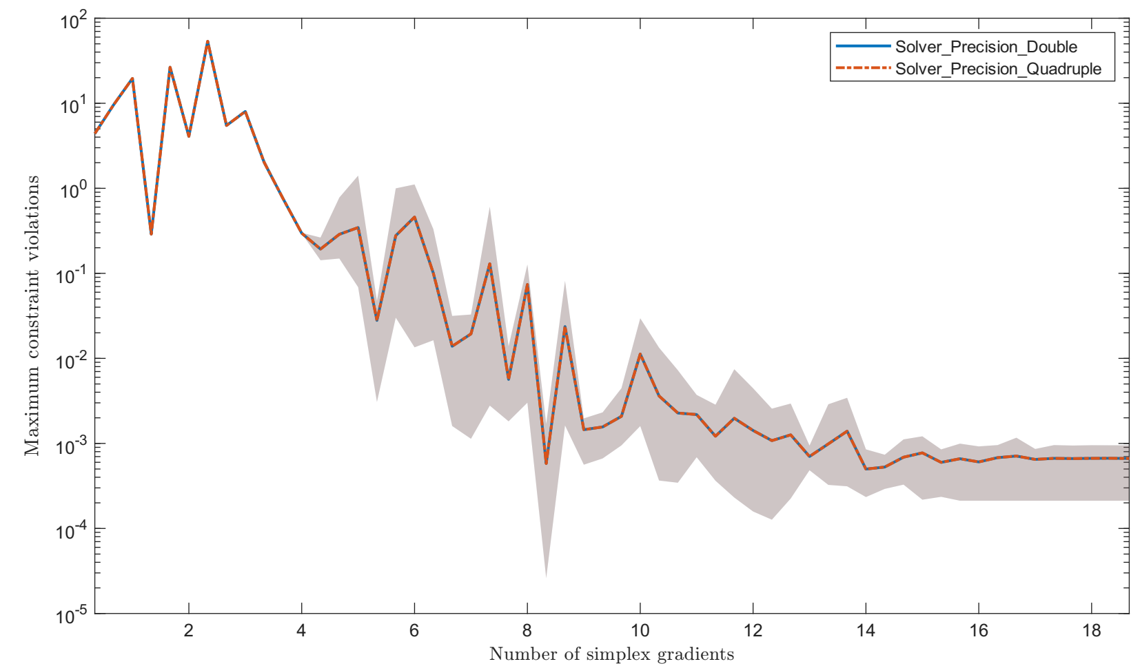
Solving "HS6" with "noisy_0.001_mixed_gaussian" feature
