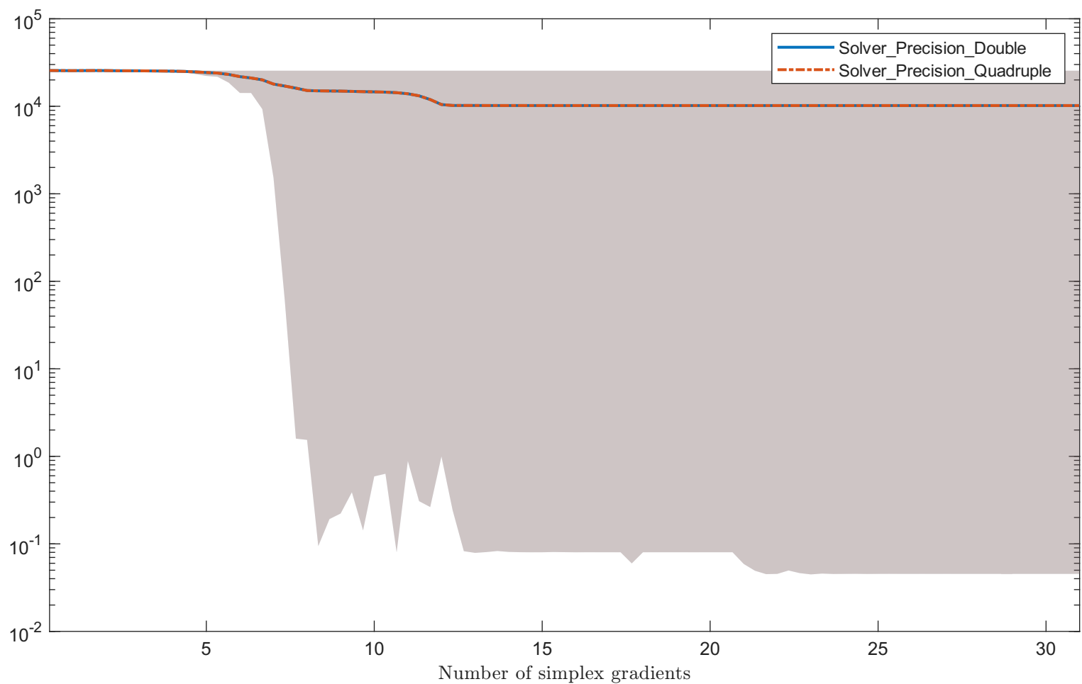
Solving "HUMPS" with "noisy_0.001_mixed_gaussian" feature
