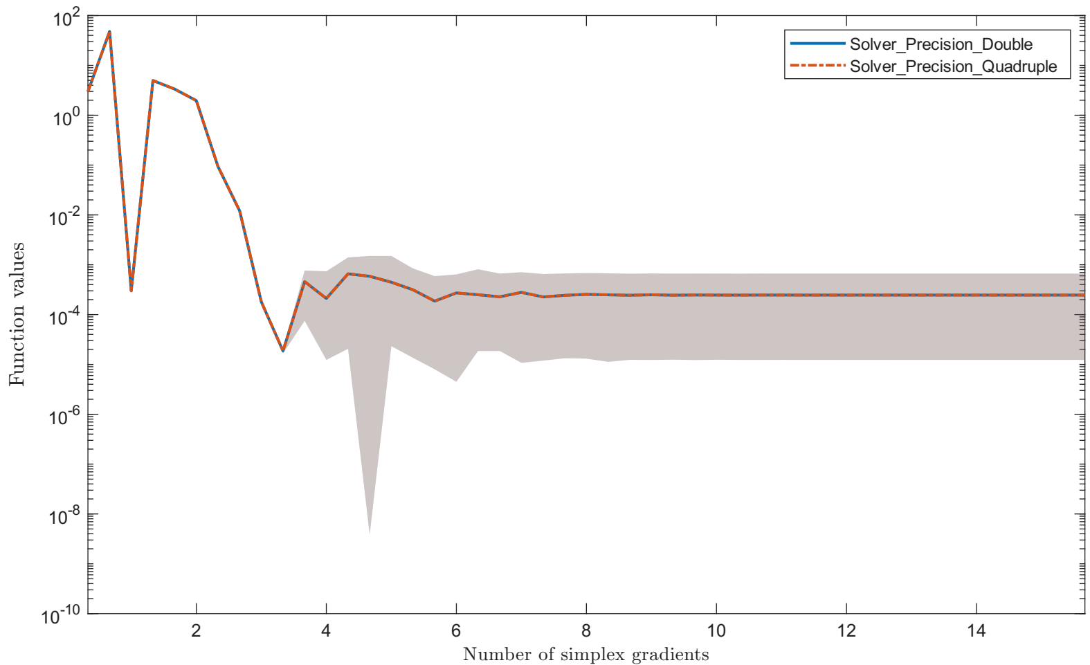
Solving "SISSER2" with "noisy_0.001_mixed_gaussian" feature
