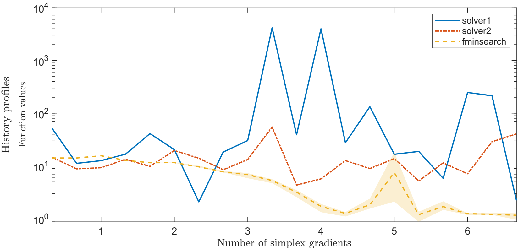
Solving "BEALE" with "noisy_0.001_mixed_gaussian" feature
