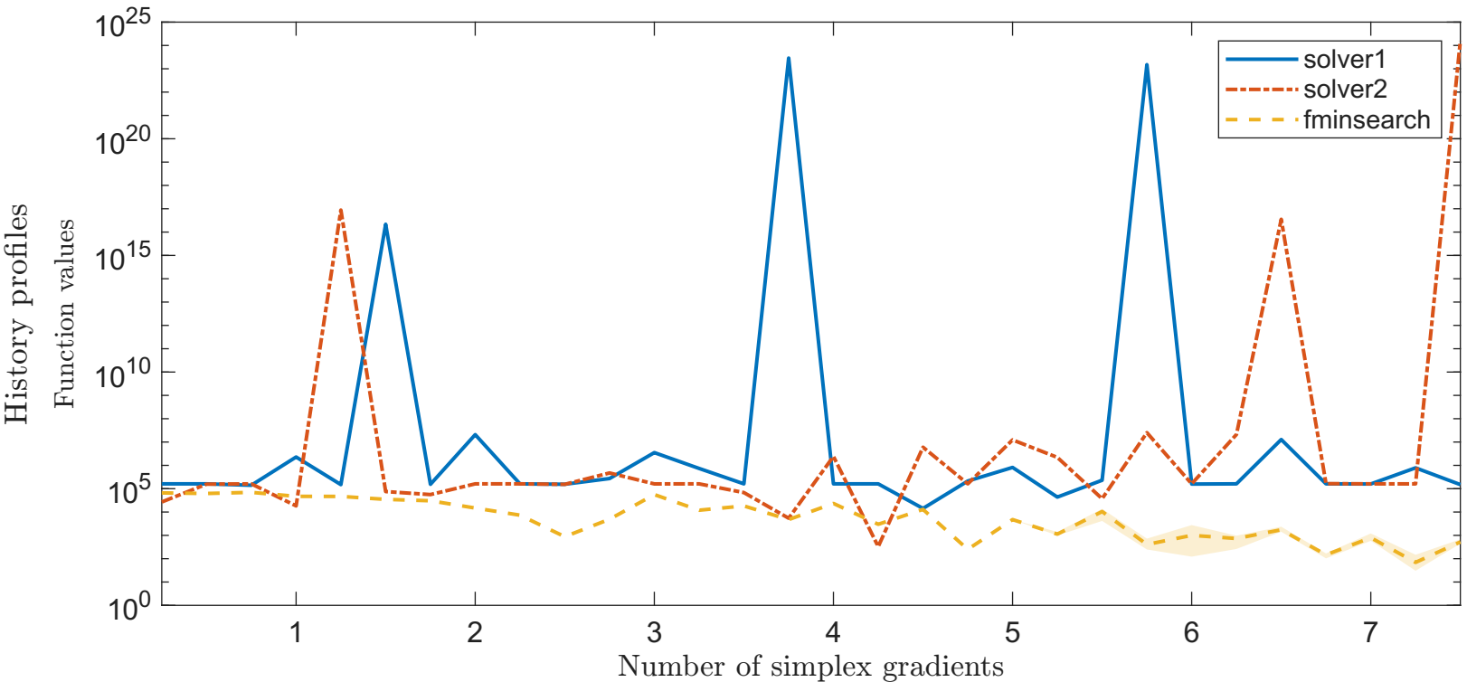
Solving "BENNETT5LS" with "noisy_0.001_mixed_gaussian" feature
