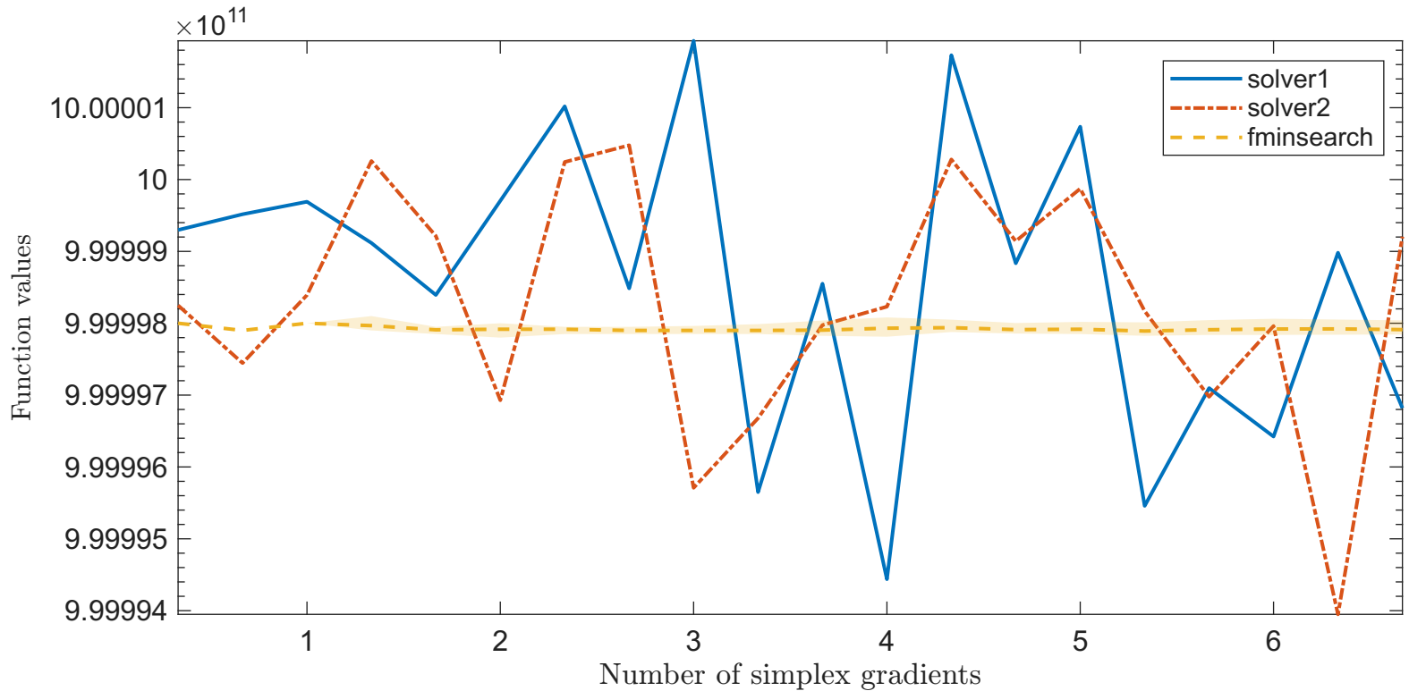
Solving "BROWNBS" with "noisy_0.001_mixed_gaussian" feature
