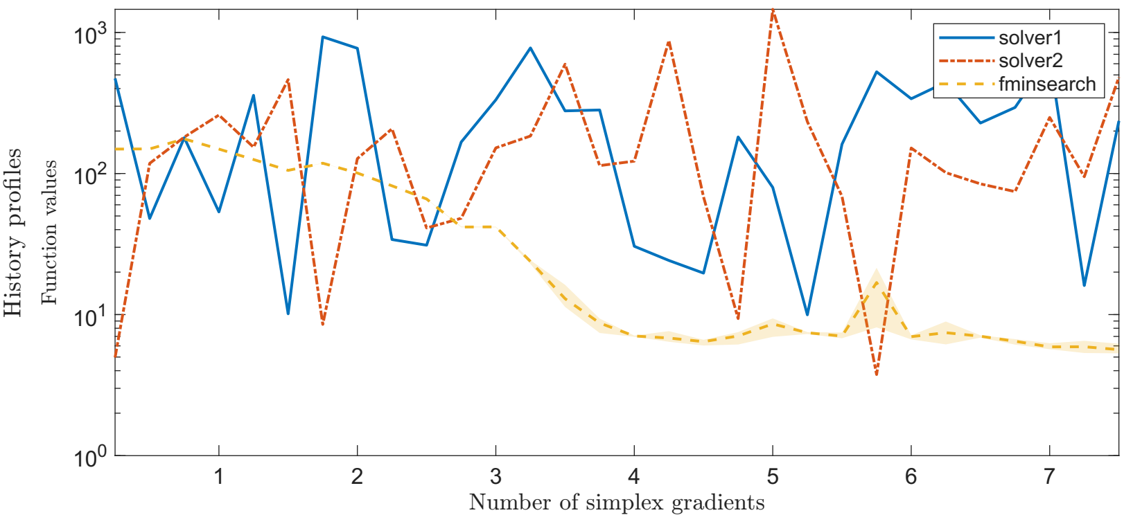
Solving "DENSCHNE" with "noisy_0.001_mixed_gaussian" feature
