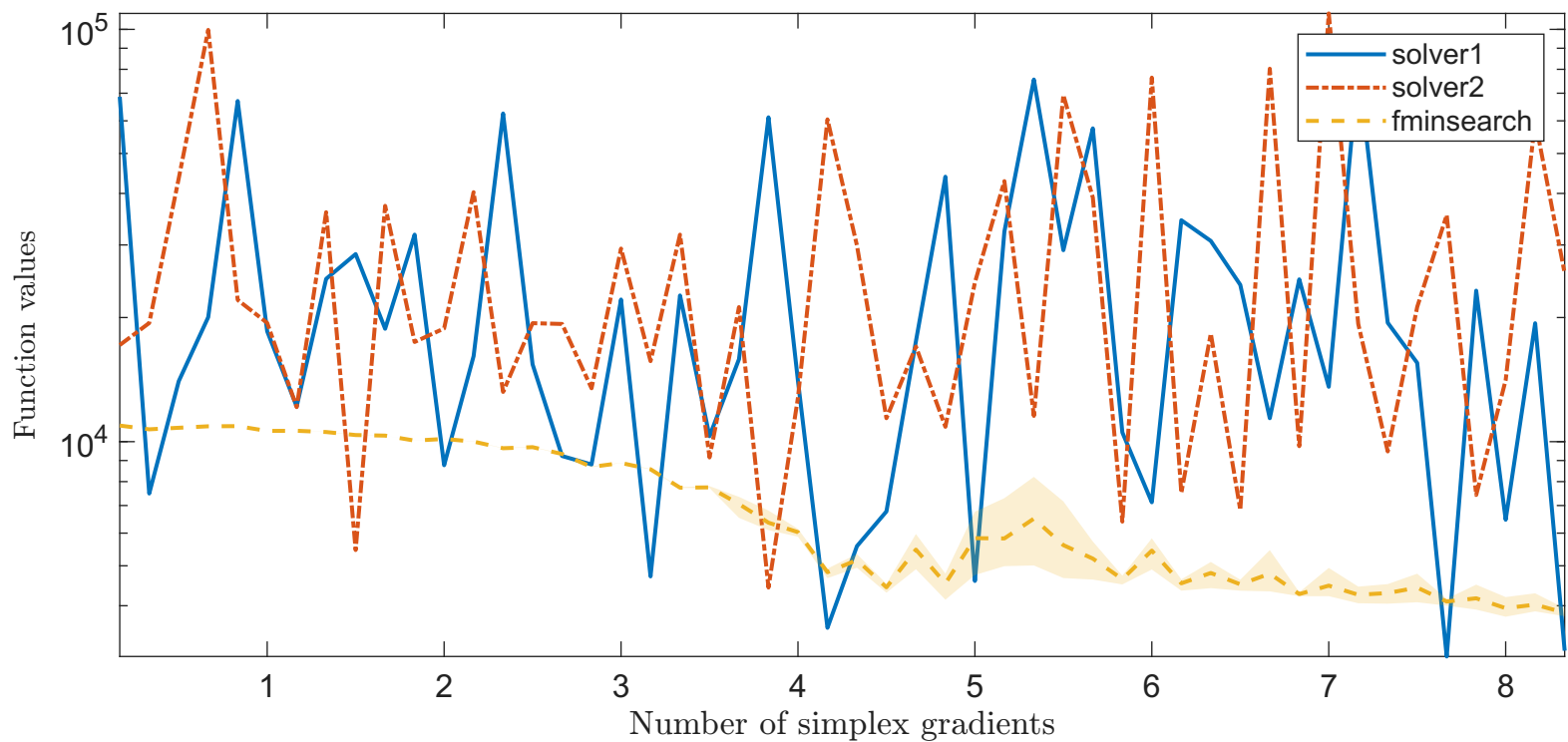
History profiles
