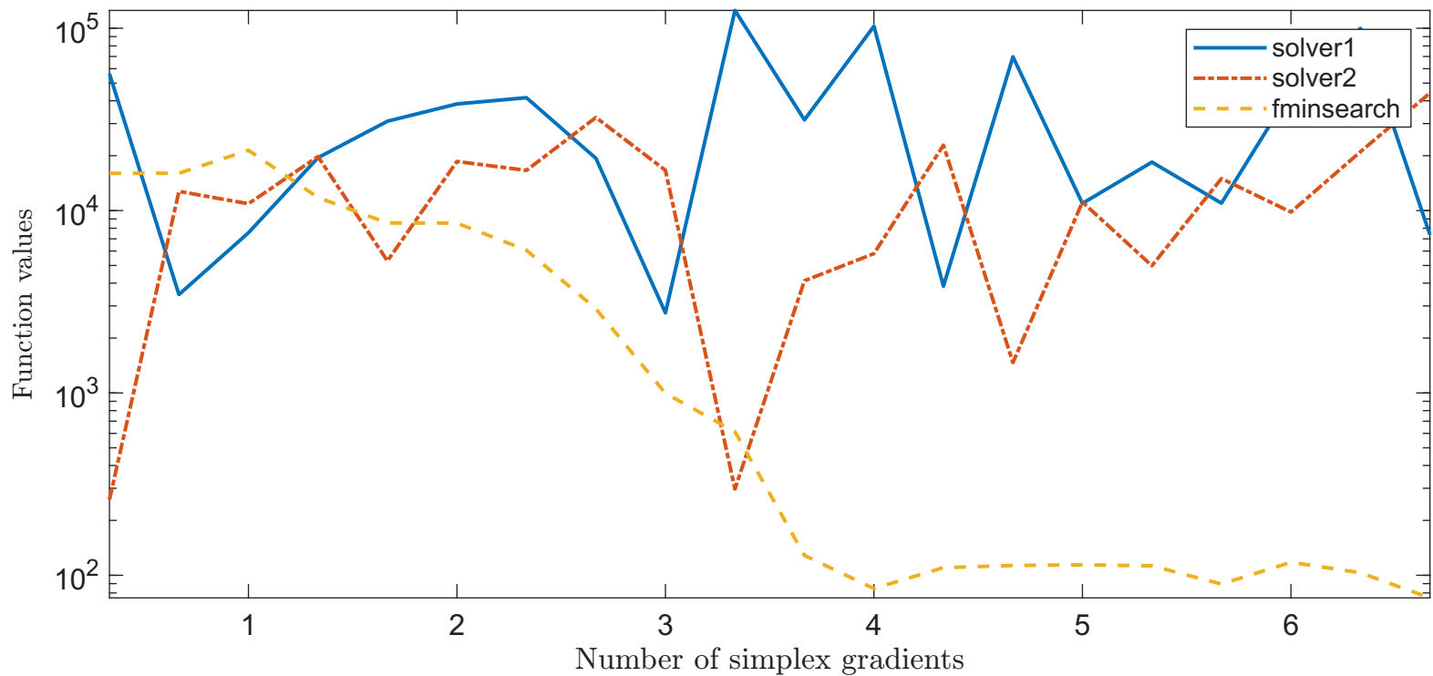
Solving "ELATVIDU" with "noisy_0.001_mixed_gaussian" feature
