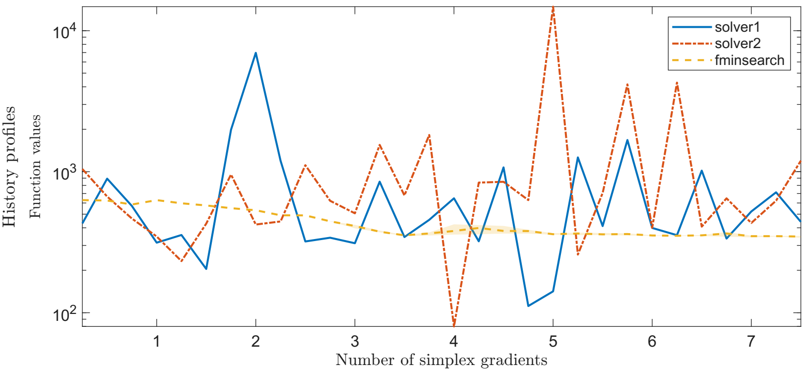
Solving “ENGVAL2” with “noisy_0.001_mixed_gaussian” feature
