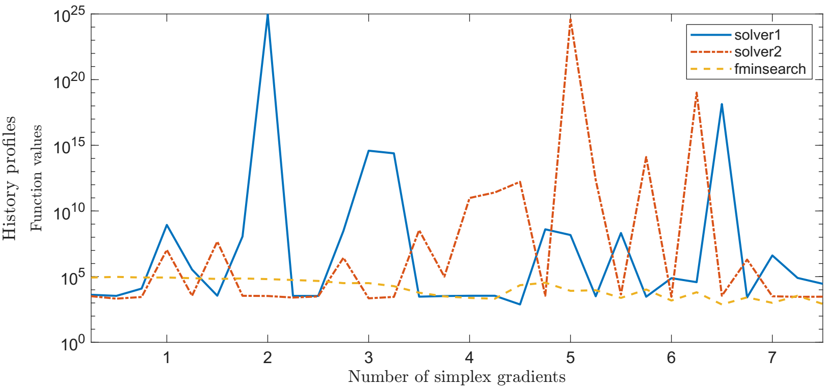
Solving "GROWTHLS" with "noisy_0.001_mixed-gaussian" feature
