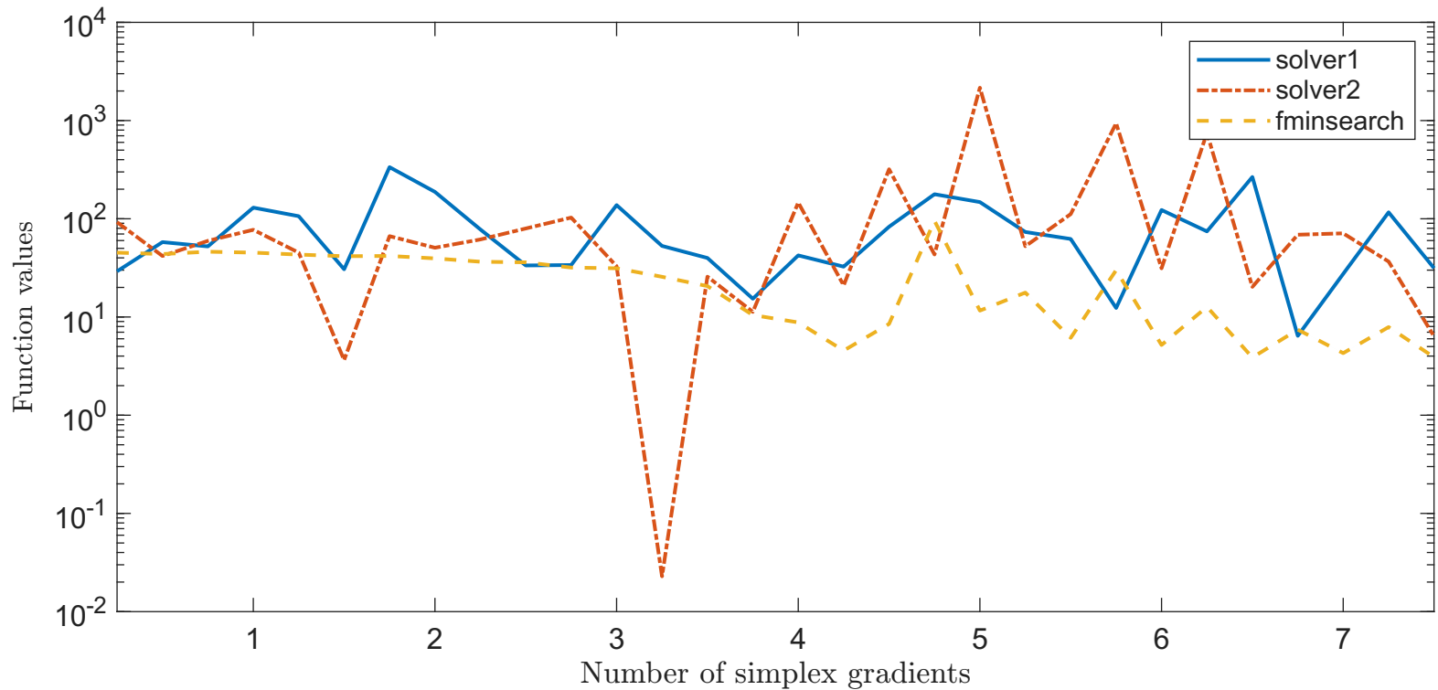
Solving "HATFLDE" with "noisy_0.001_mixed_gaussian" feature
