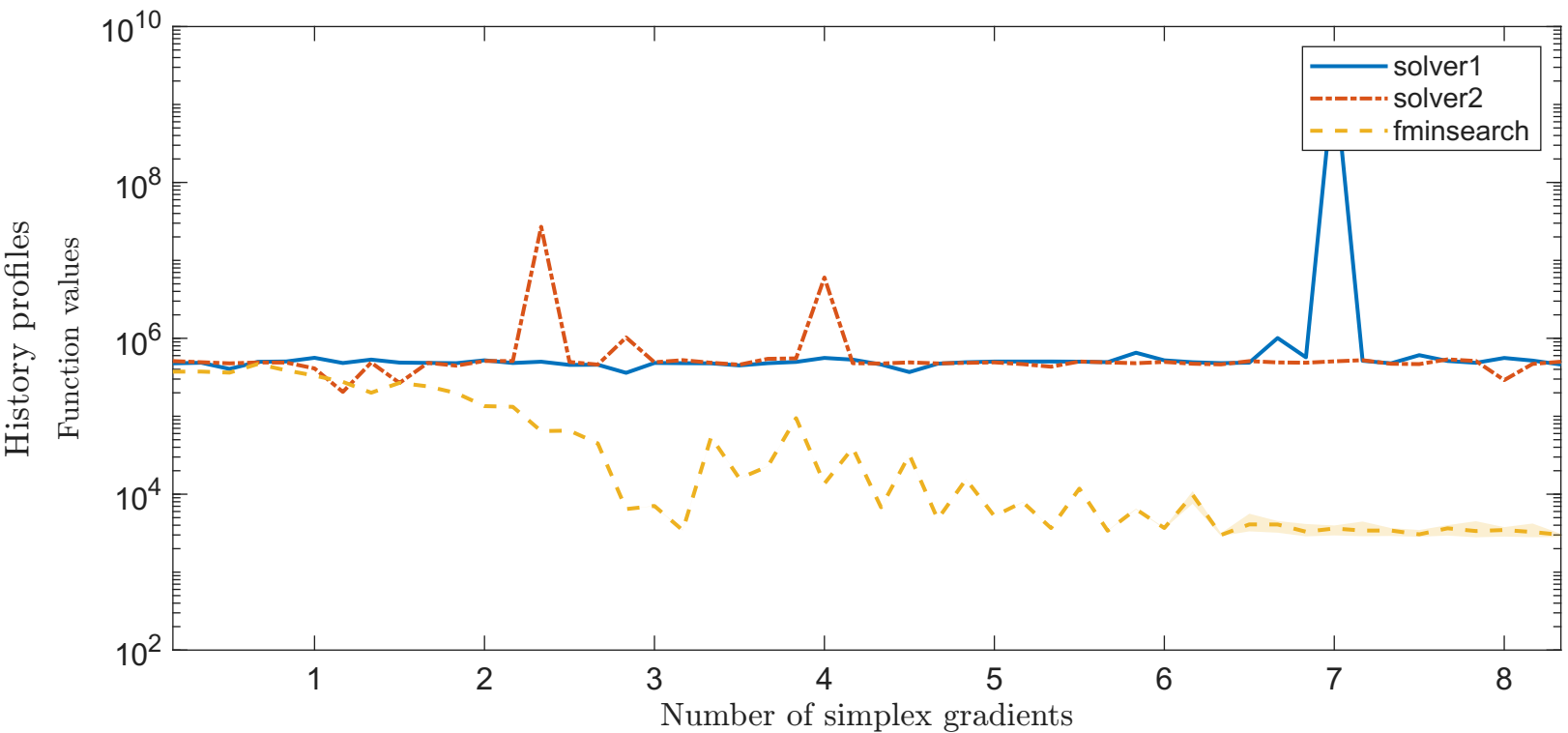
Solving "KIRBY2LS" with "noisy_0.001_mixed_gaussian" feature
