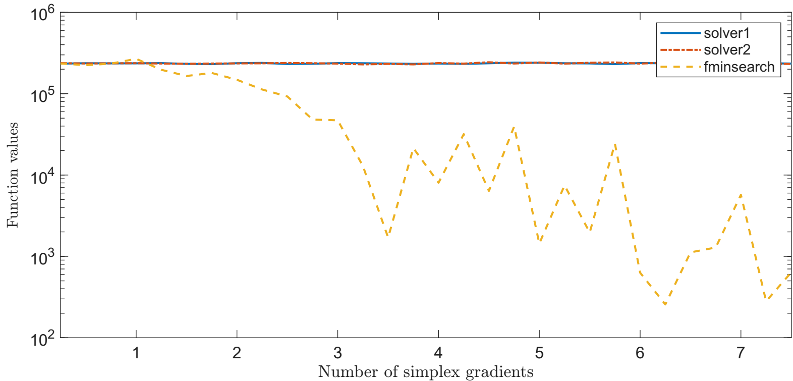
Solving "LSC2LS" with "noisy_0.001_mixed_gaussian" feature
