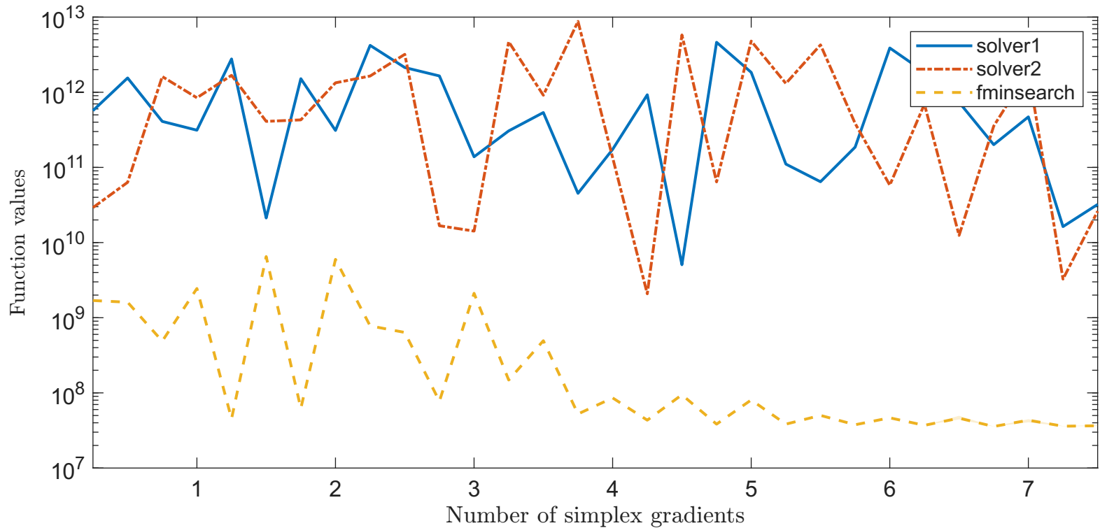
Solving "MEYER3" with "noisy_0.001_mixed_gaussian" feature
