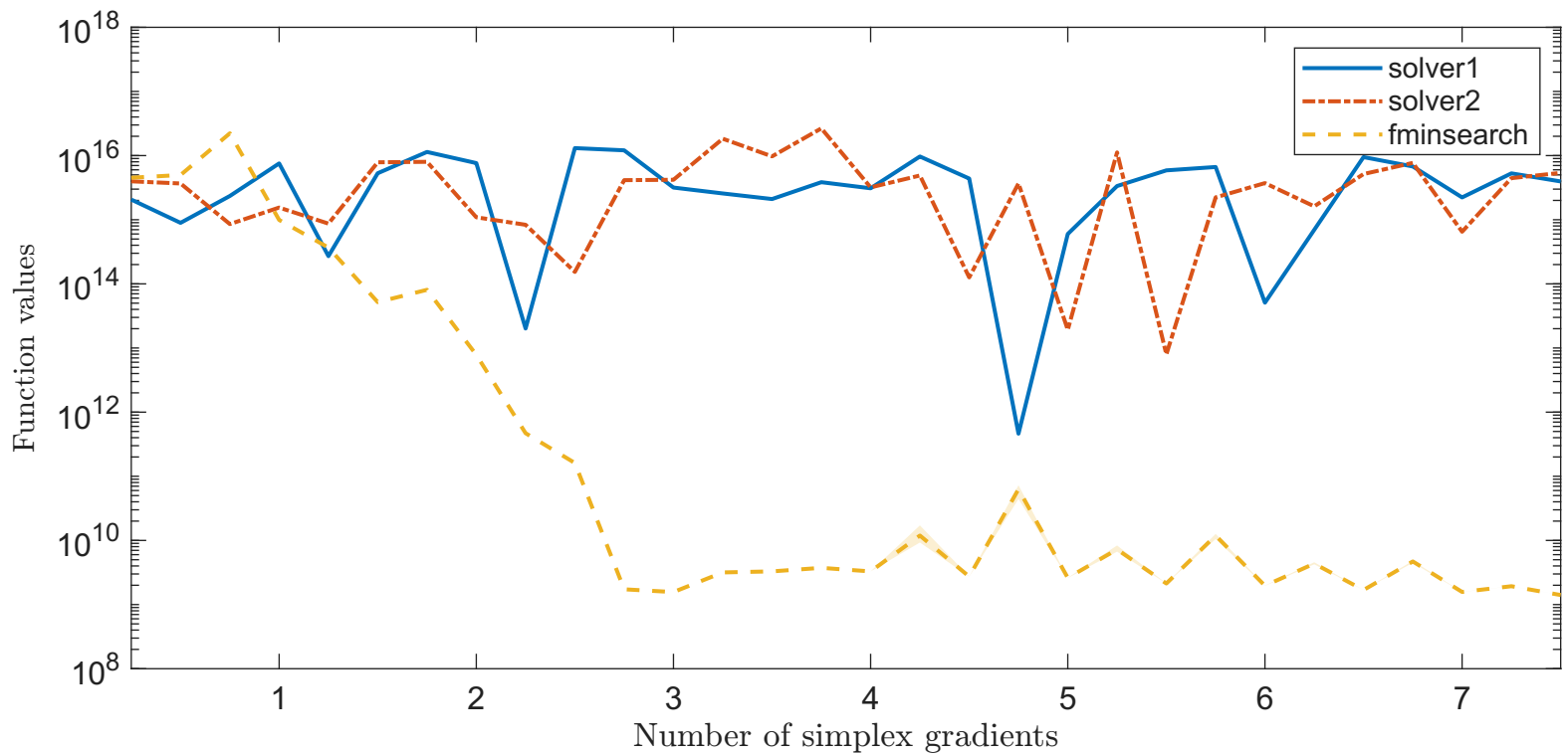
Solving "MGH10LS" with "noisy_0.001_mixed_gaussian" feature
