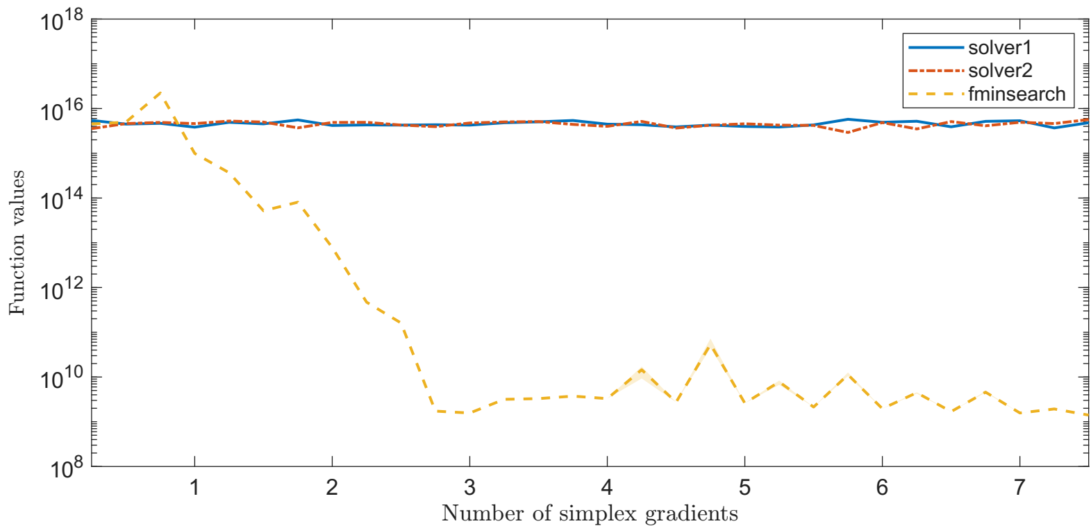
Solving “MGH10SLS” with “noisy_0.001_mixed_gaussian” feature
