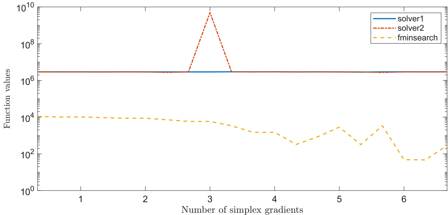
Solving “MISRA1BLS” with “noisy_0.001_mixed.gaussian” feature
