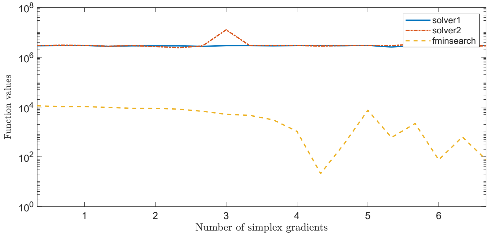
Solving "MISRA1DLS" with "noisy_0.001_mixed_gaussian" feature
