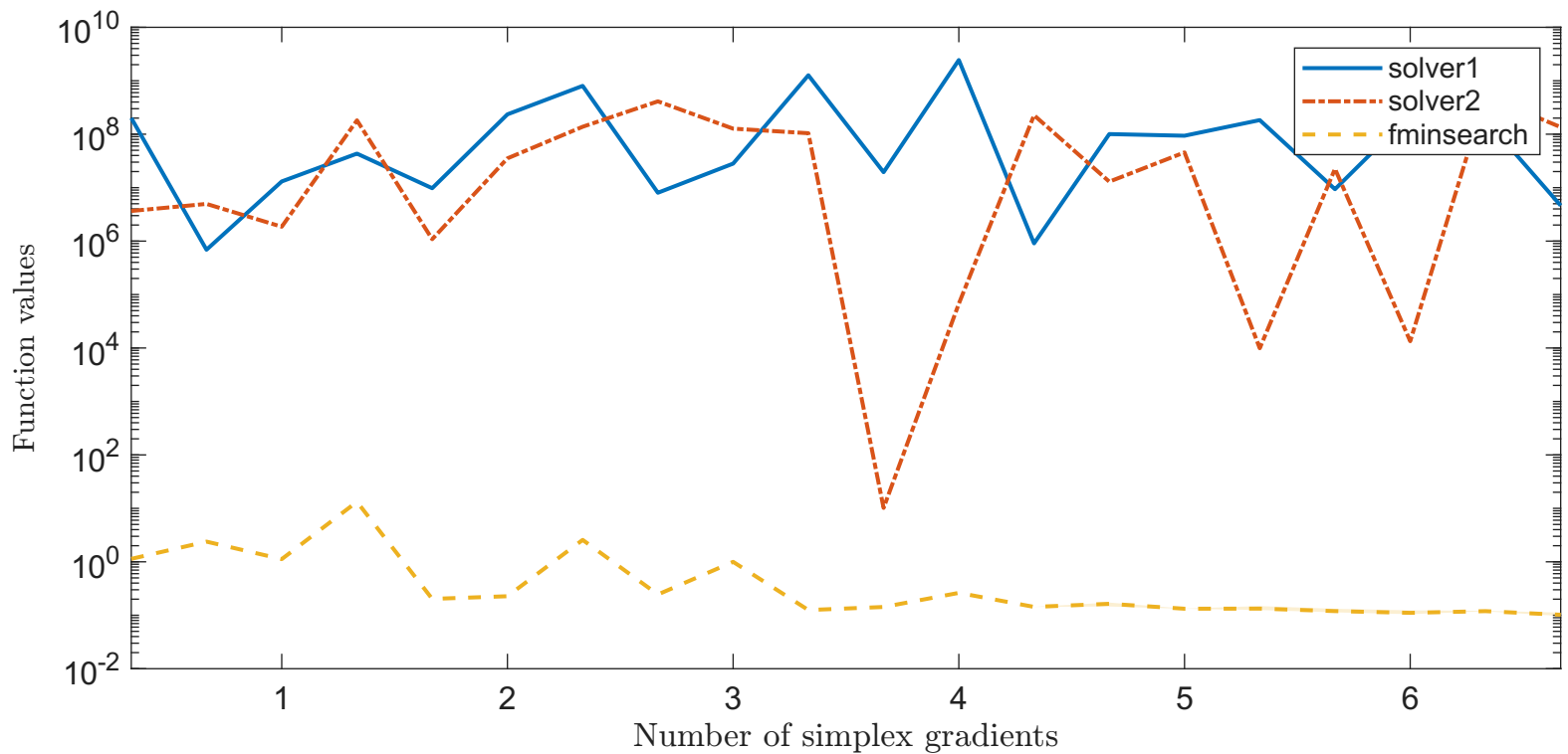
Solving "POWELLBSLS" with "noisy_0.001_mixed_gaussian" feature
