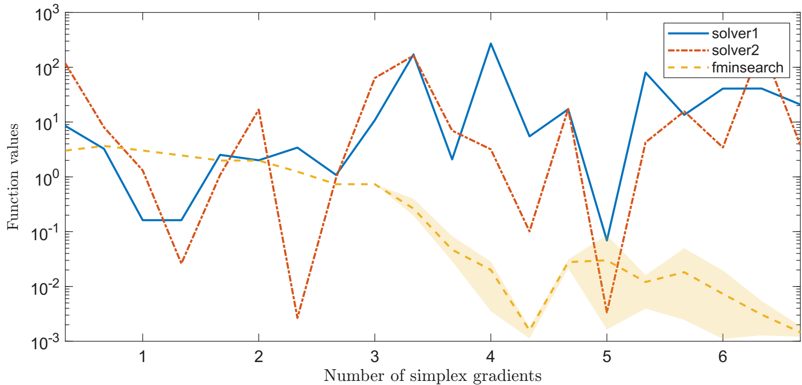
Solving "SISSER" with "noisy_0.001_mixed_gaussian" feature
