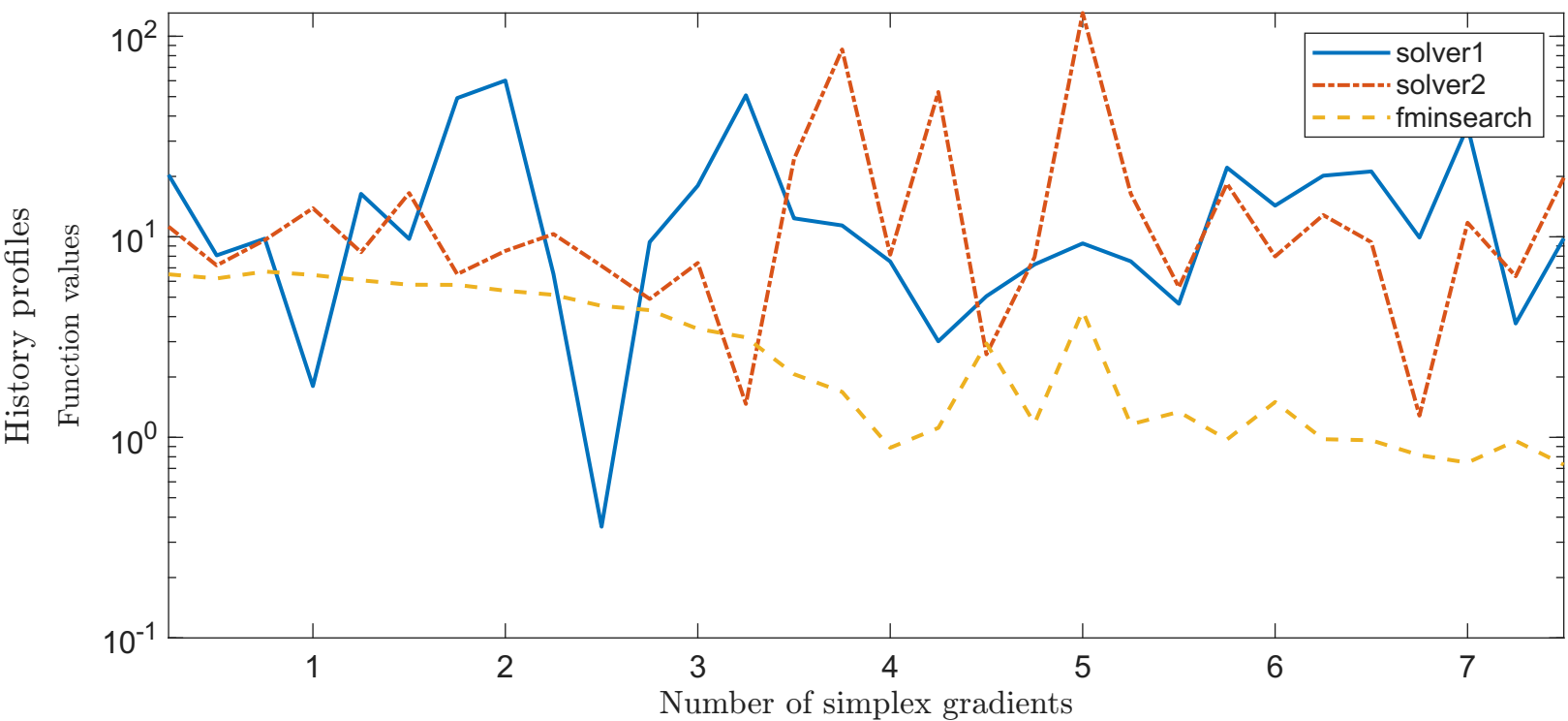
Solving "SSI" with "noisy_0.001_mixed_gaussian" feature
