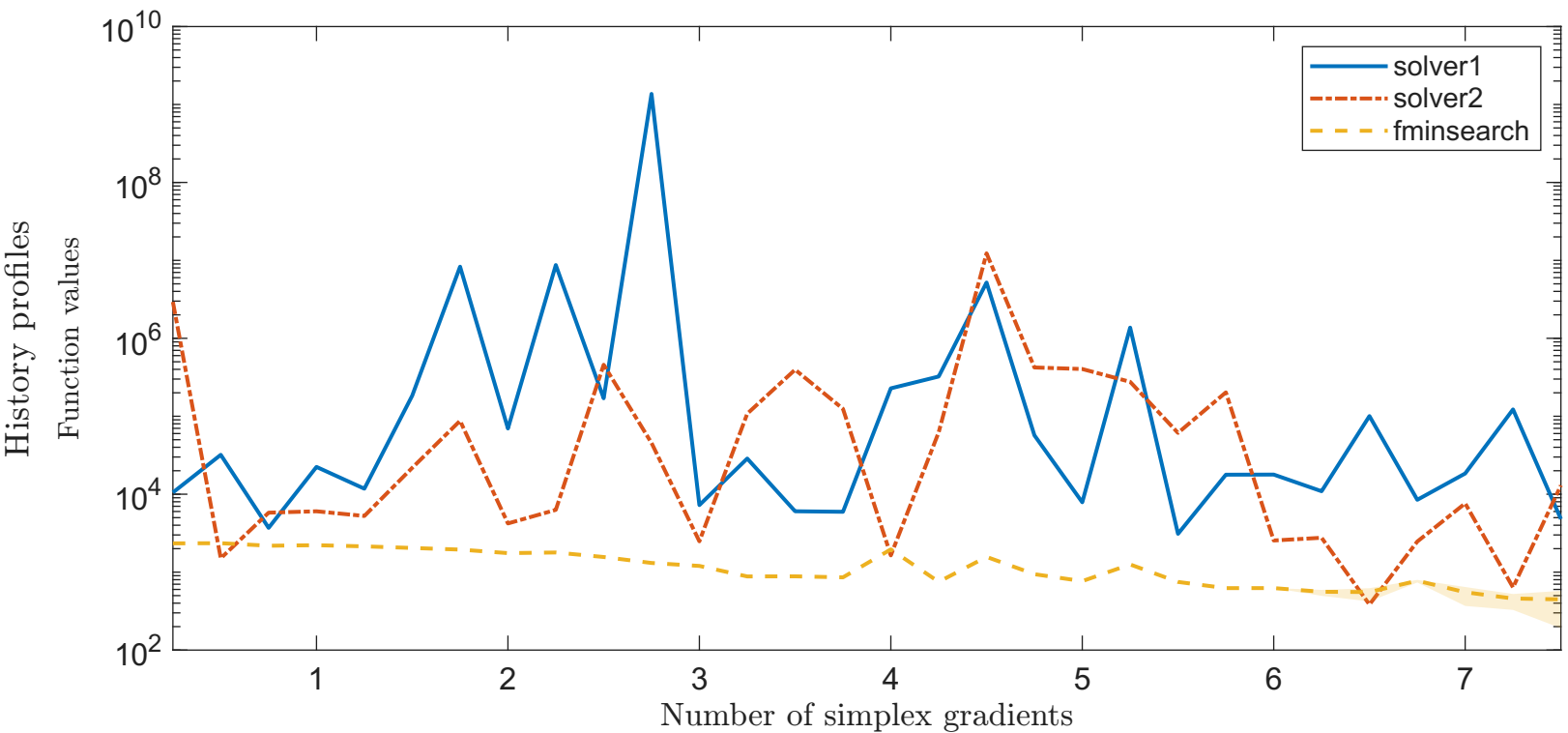
Solving “YFITU” with “noisy_0.001_mixed_gaussian” feature
