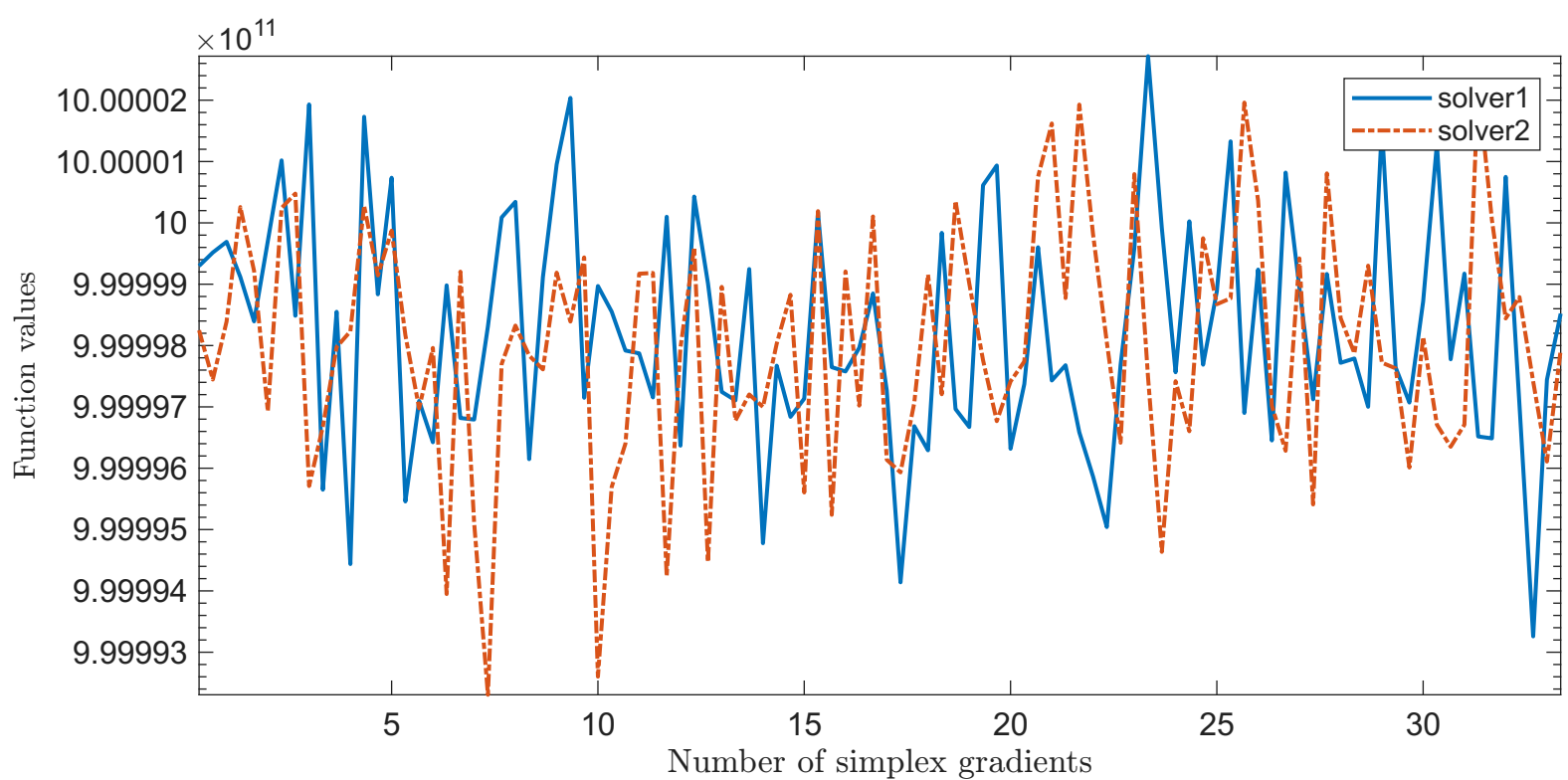
Solving "BROWNBS" with "plain" feature
