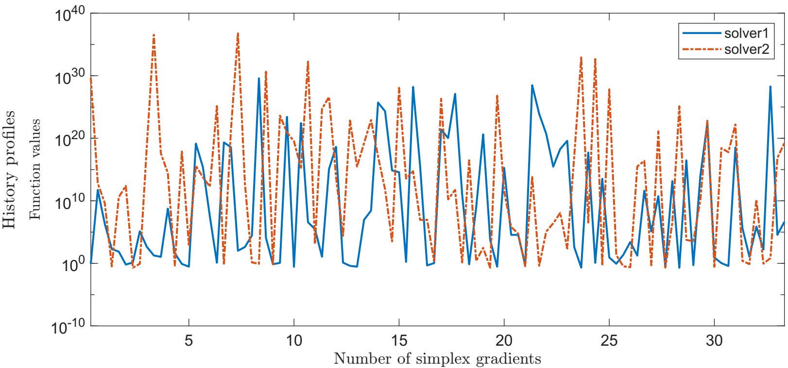
Solving "CLIFF" with "plain" feature
