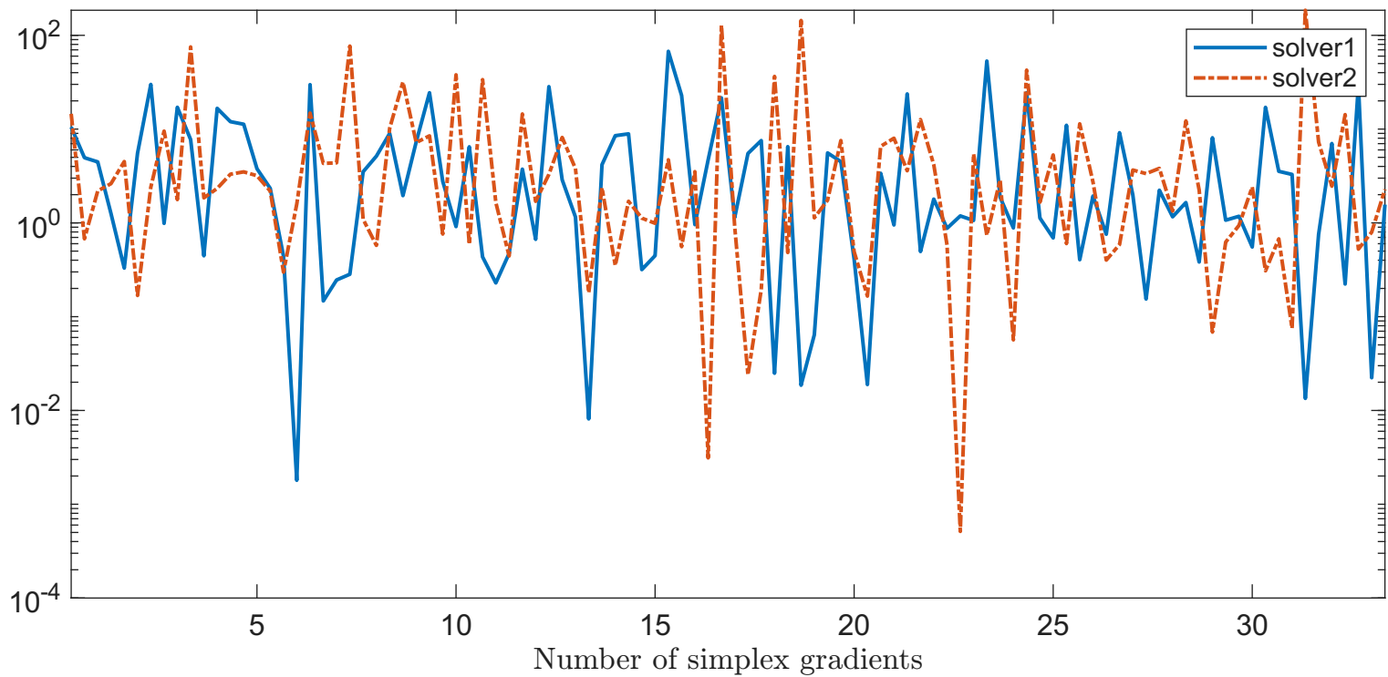
Solving "CLUSTERLS" with "plain" feature
