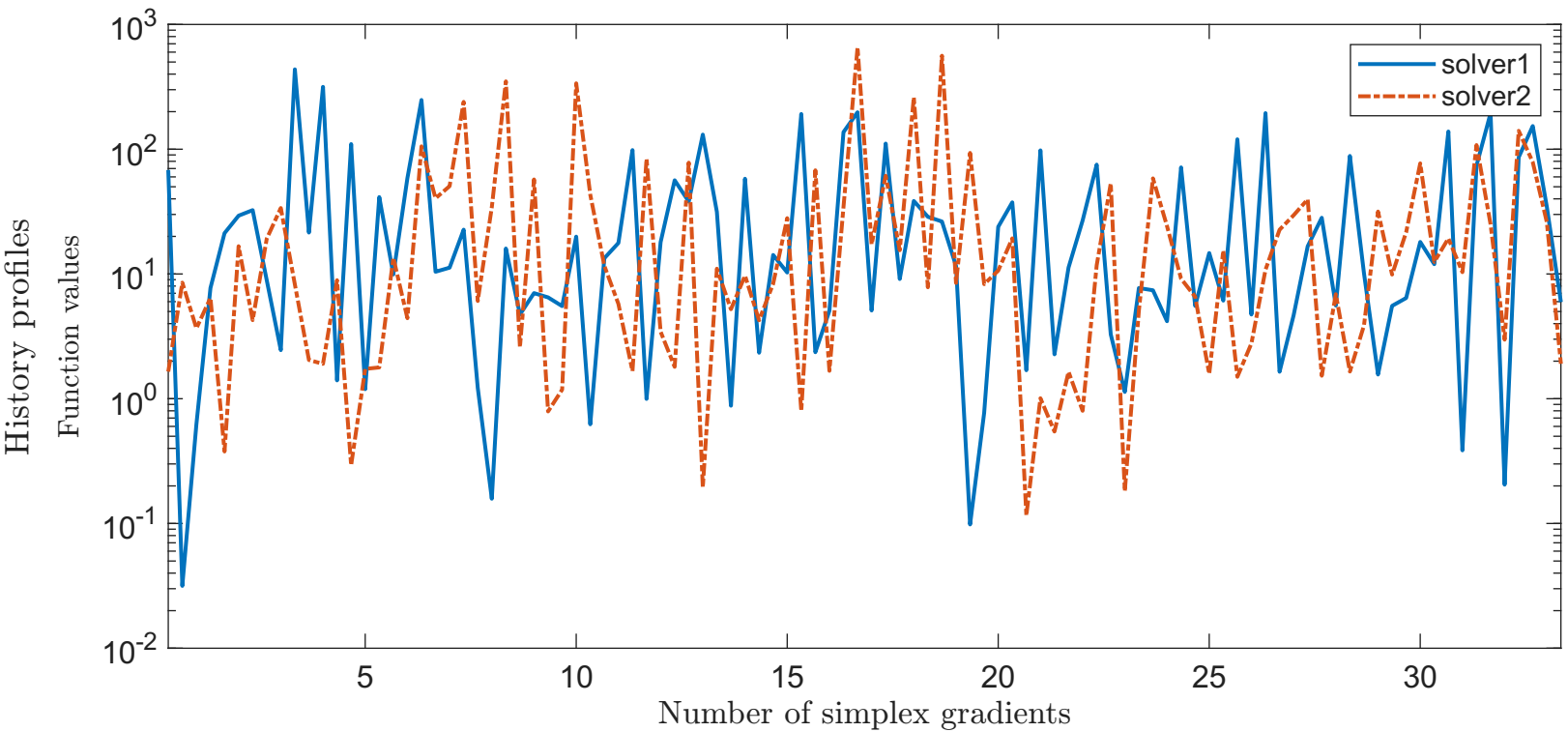
Solving "DENSCHNA" with "plain" feature
