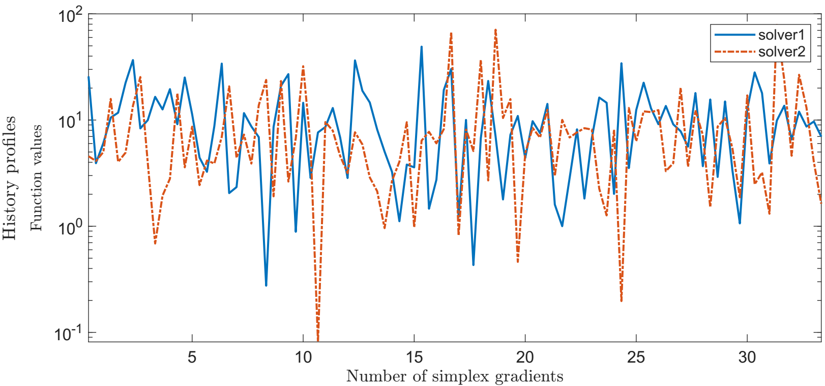
Solving "DENSCHNB" with "plain" feature
