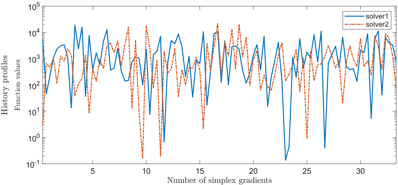
Solving "DENSCHNC" with "plain" feature
