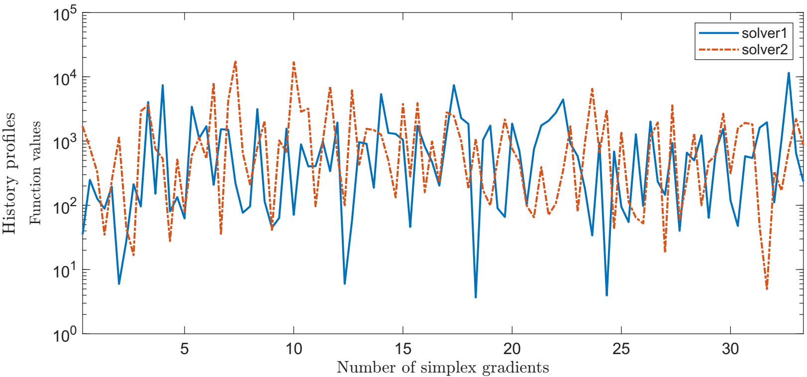
Solving "DENSCHNF" with "plain" feature
