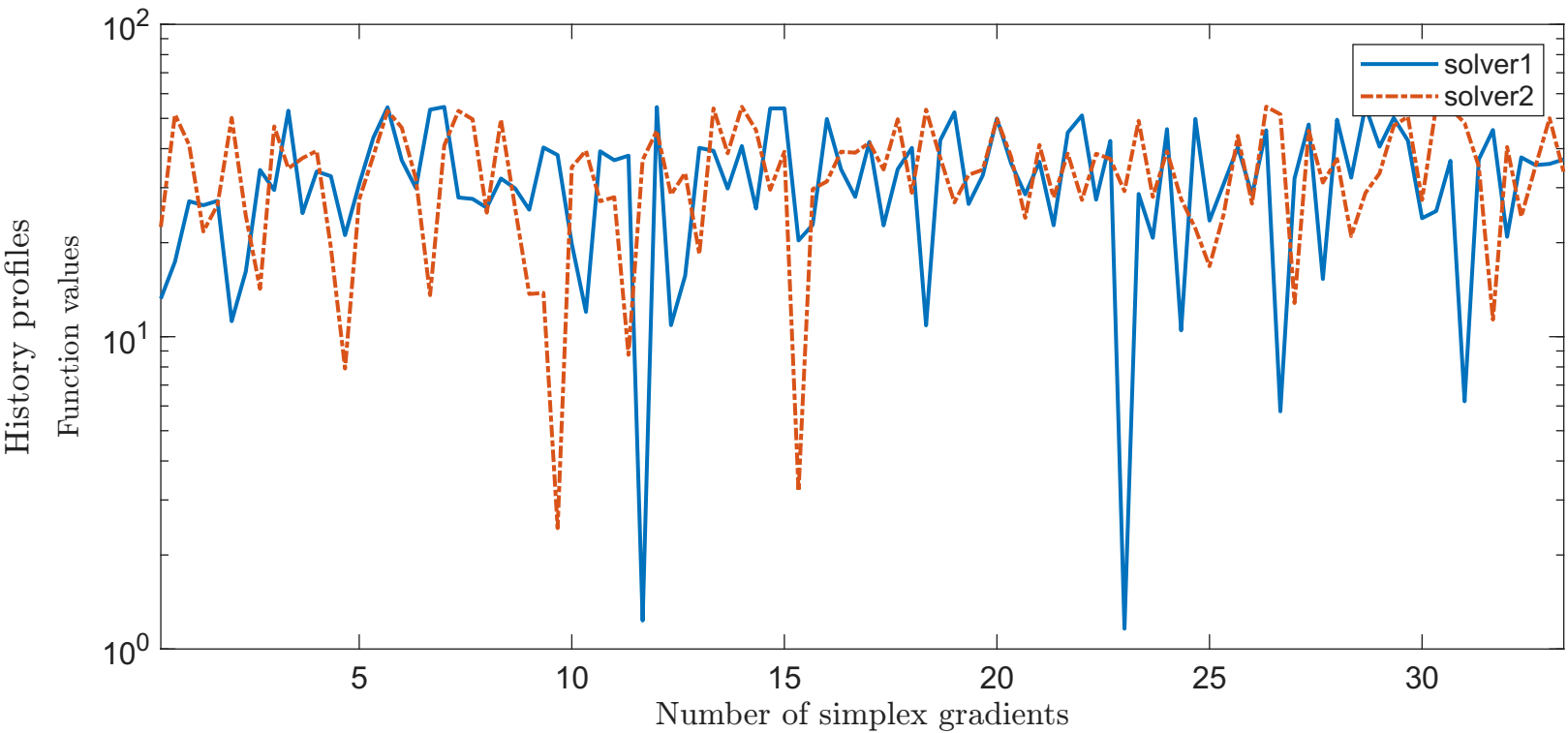
Solving "EGGCRAVE" with "plain" feature
