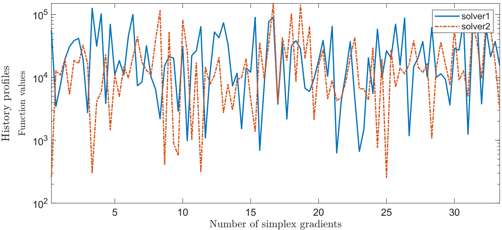
Solving "ELATVIDU" with "plain" feature
