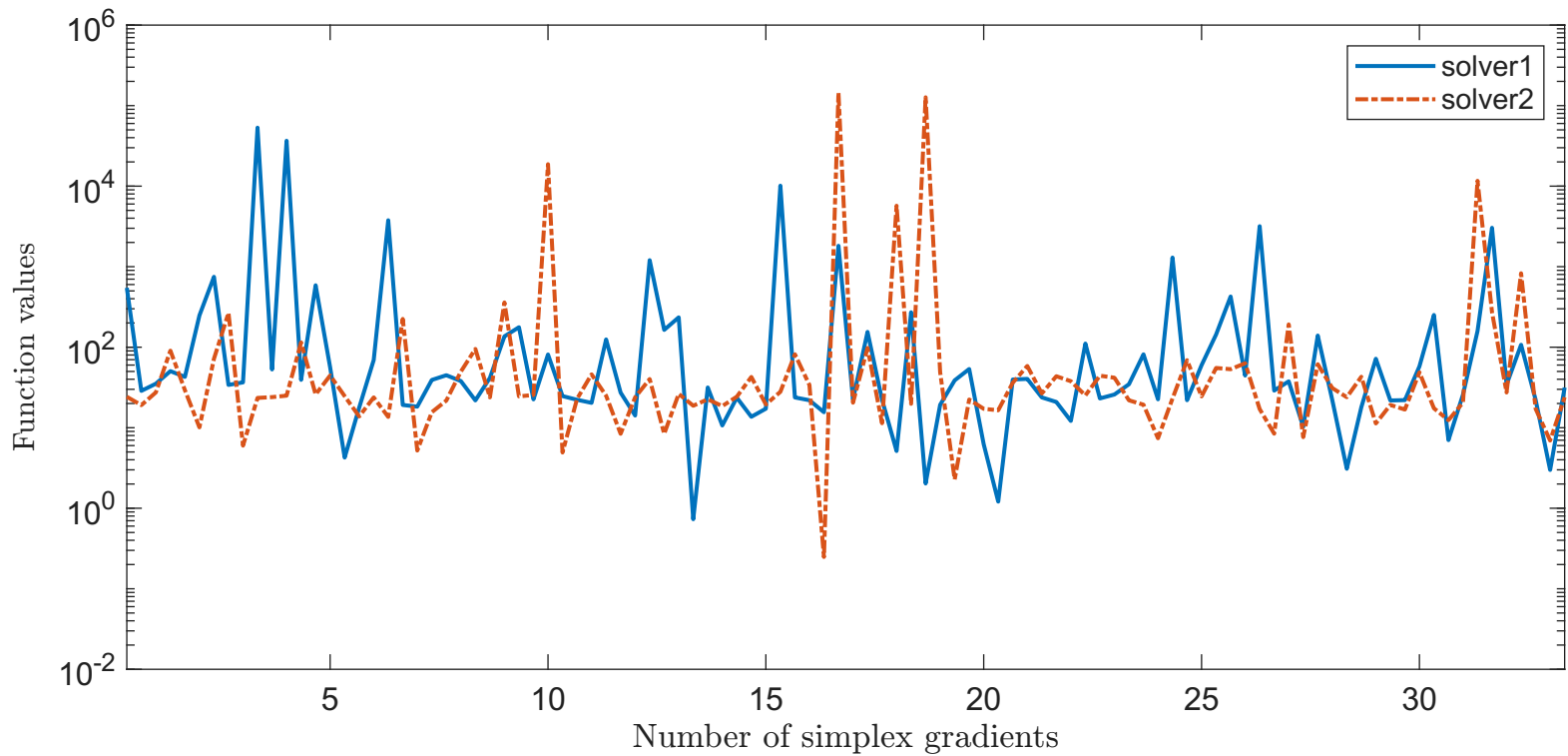
Solving "EXPFIT" with "plain" feature
