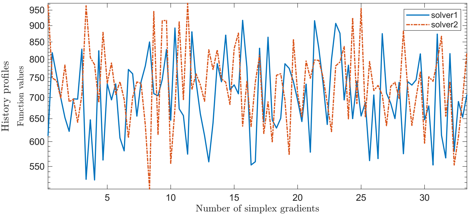
Solving "HAIRY" with "plain" feature
