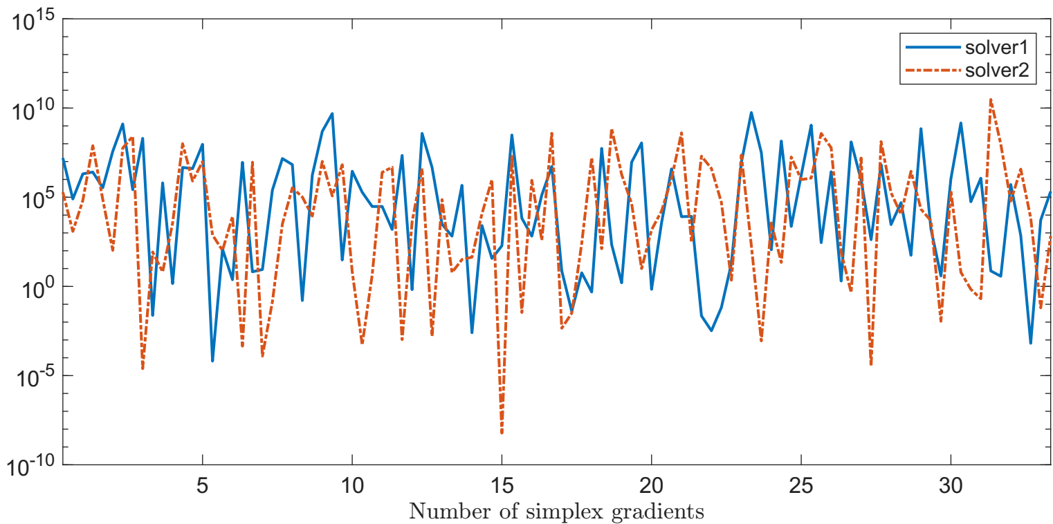
Solving "HIMMELBB" with "plain" feature
