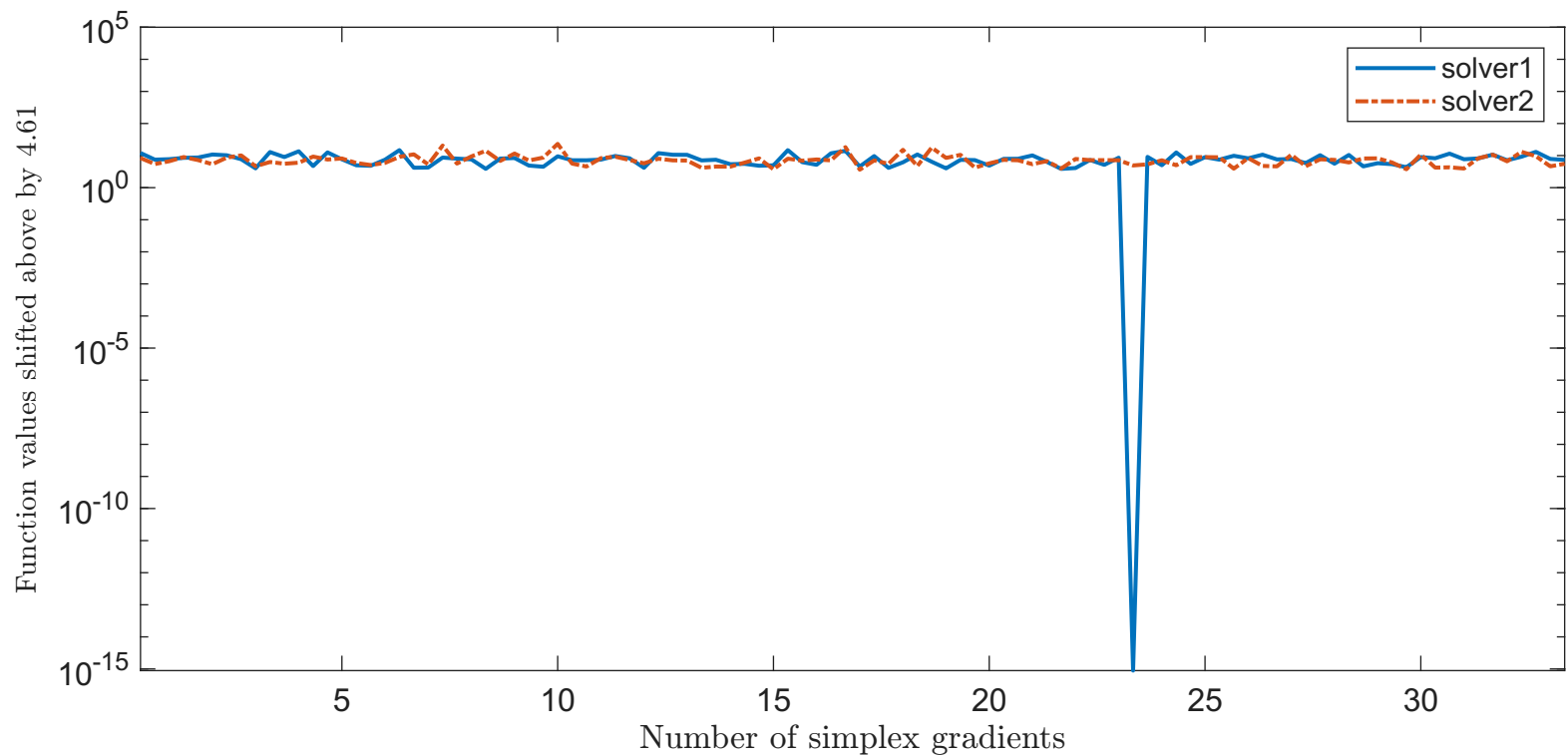
Solving "HIMMELBH" with "plain" feature
