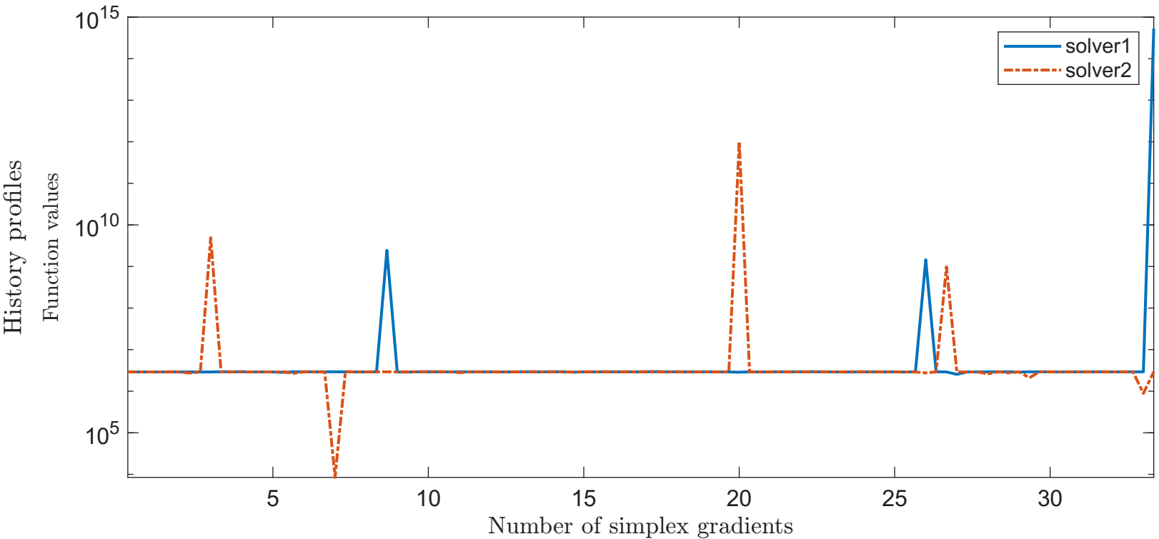
Solving "MISRA1BLS" with "plain" feature
