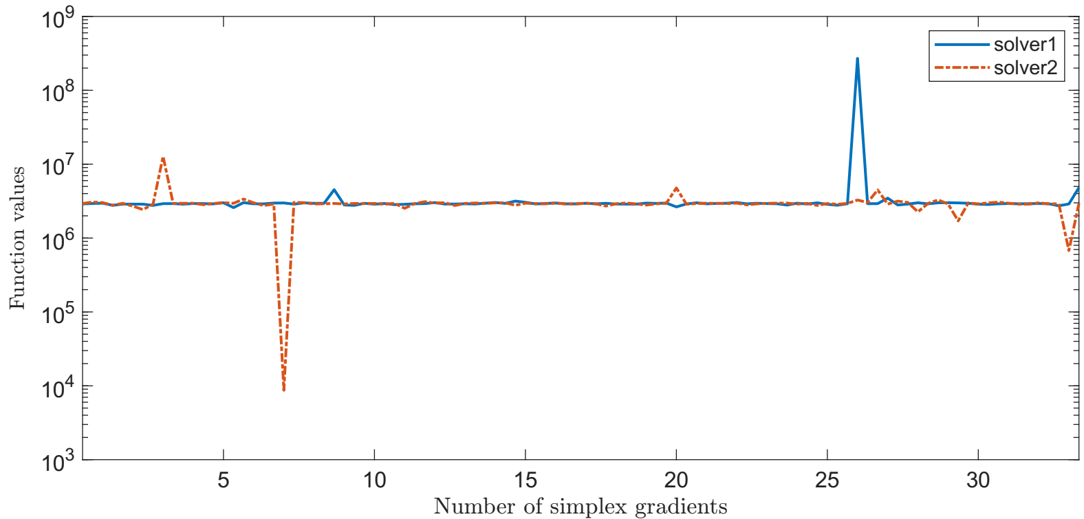
Solving "MISRA1DLS" with "plain" feature
