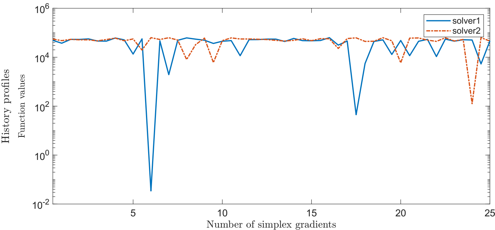
Solving "MUONSINELS" with "plain" feature
