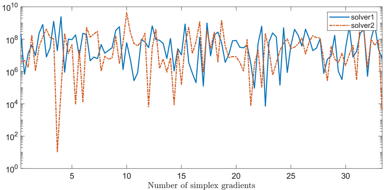
Solving "POWELLBLS" with "plain" feature
