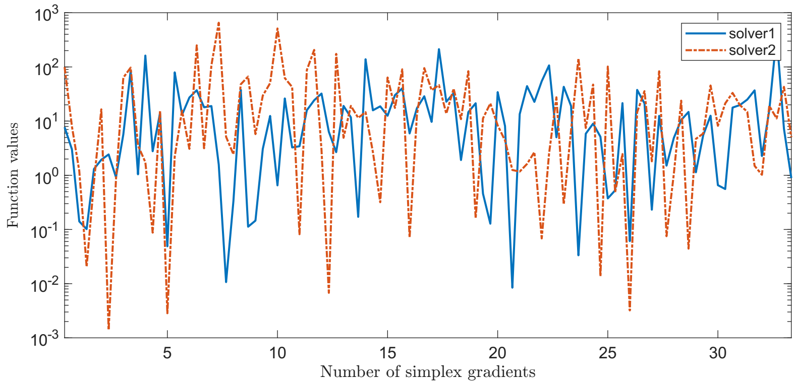
Solving "SISSER2" with "plain" feature
