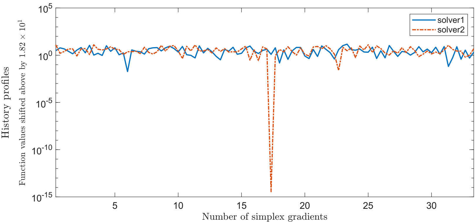
Solving “ZANGWIL2” with “plain” feature
