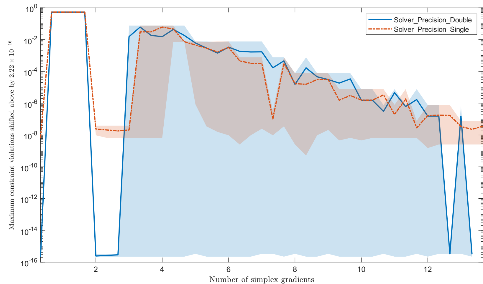
Solving "ALSOTAME" with "noisy_0.001_mixed_gaussian" feature
