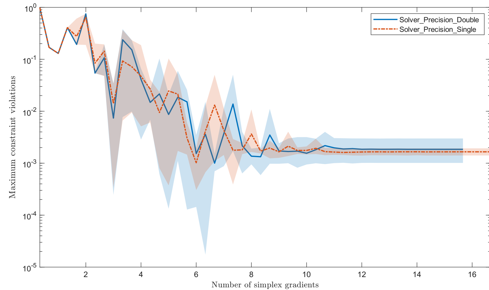
Solving "BT1" with "noisy_0.001_mixed_gaussian" feature
