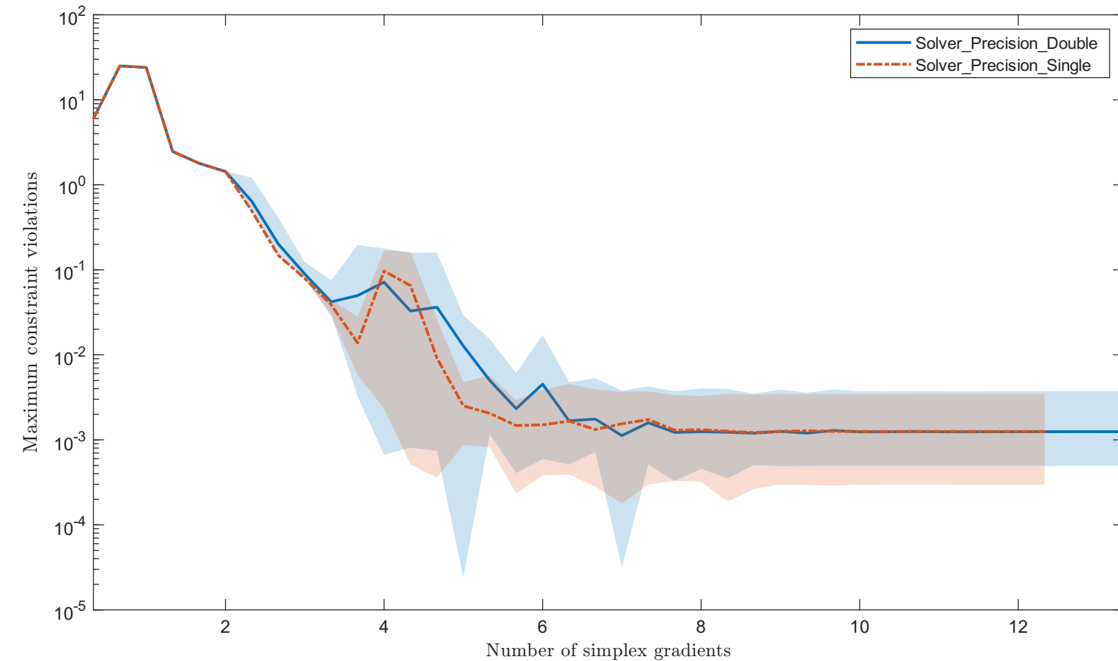
Solving "BT10" with "noisy_0.001_mixed_gaussian" feature
