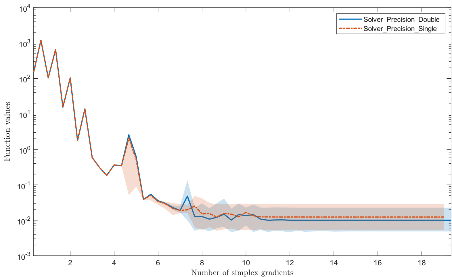
Solving “DANIWOODLS” with “noisy_0.001_mixed_gaussian” feature
