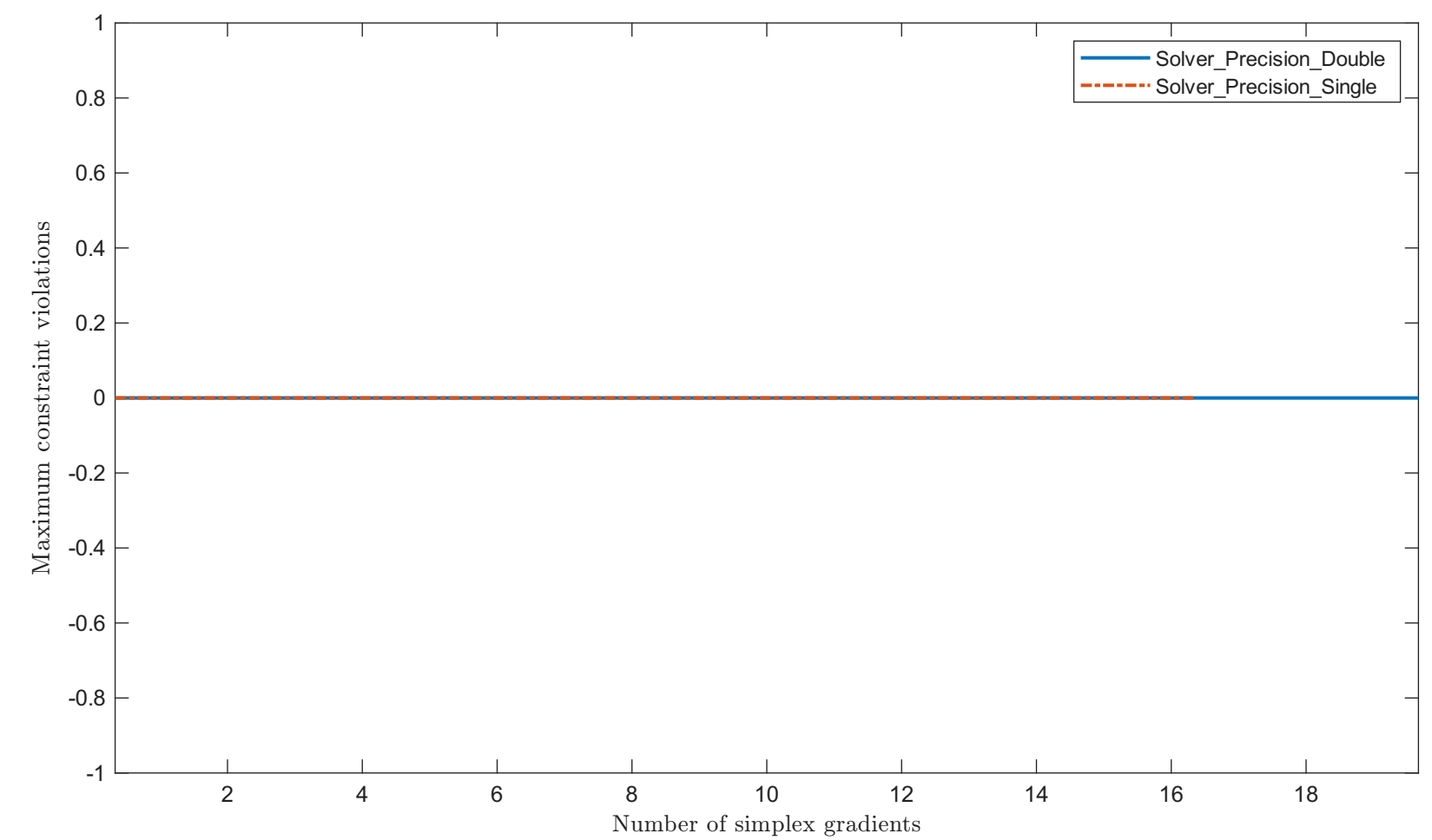
Solving “EXP2B” with “noisy_0.001_mixed_gaussian” feature
