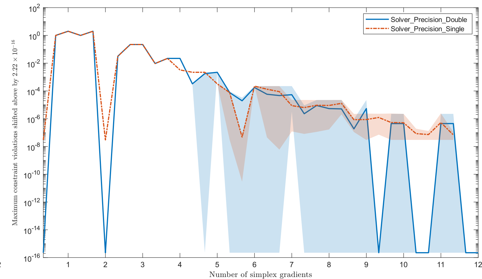
Solving “EXTRASIM” with “noisy_0.001_mixed_gaussian” feature
