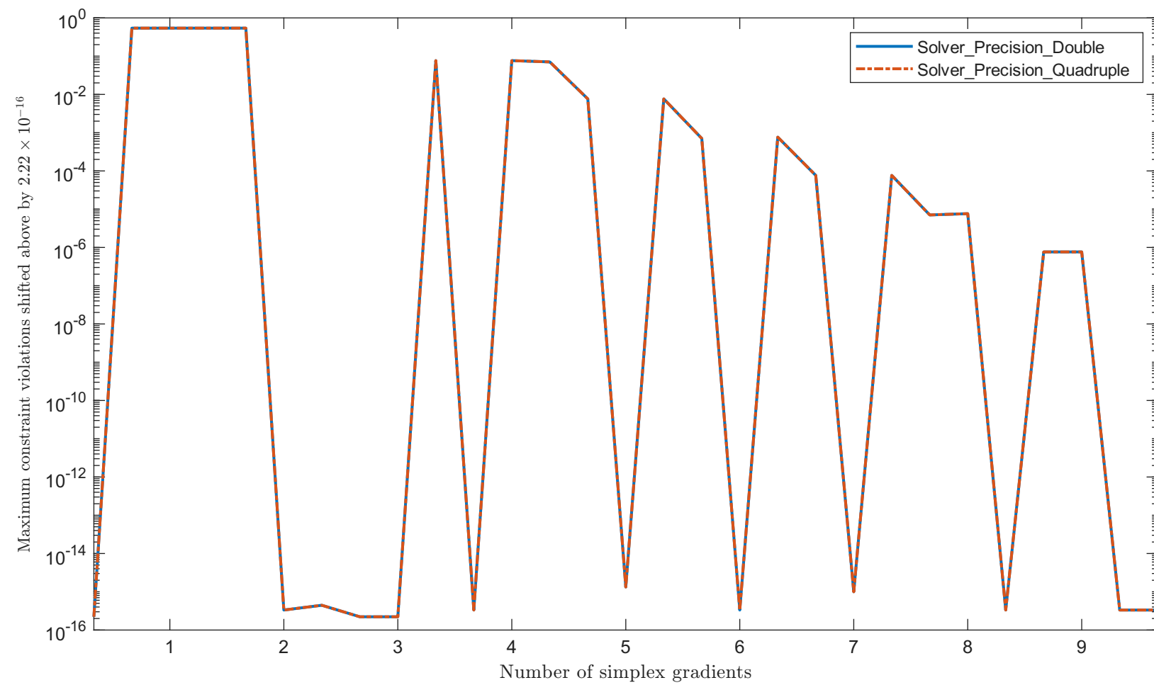
Solving "ALSOTAME" with "plain" feature
