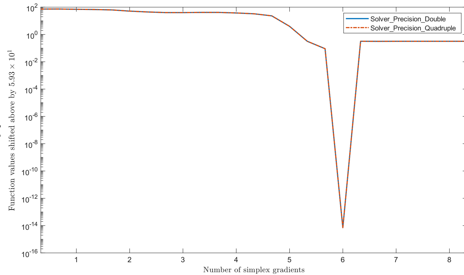
History profiles
